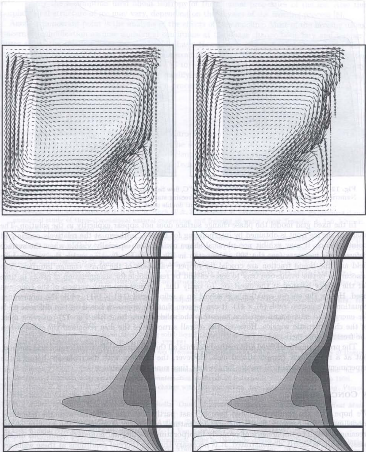
Fig. 11. Freezing of water: T_h = 10^\circ\text{C} , T_c = -10^\circ\text{C} . Numerical solutions (FGM) obtained at 120's (left column) and 500's (right) after freezing starts from the steady convective flow. Velocity vectors (top row) and temperature fields (bottom) displayed
