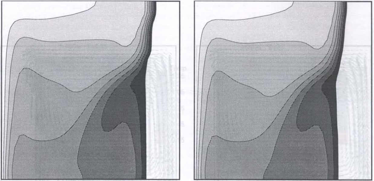
Fig. 12. Freezing of water for T_h = 10^\circ\text{C} , T_c = -10^\circ\text{C} , flow field calculated for adiabatic boundary condition. Numerical solutions (FGM) obtained at 500 s after freezing starts from the steady convective flow; left: single mesh; right: double mesh
