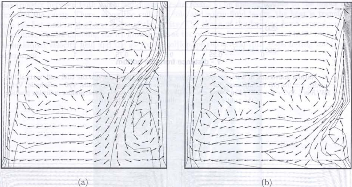
Fig. 5. Natural convection of water, 3D numerical results (FRE) for T_h = 10^\circ\text{C} , T_c = 0^\circ . Velocity and temperature fields in the centre plane ( z = 0.5 ). Effect of TBC; (a) – adiabatic TBC, (b) – non-adiabatic 1D-TBC with heat transfer coefficient h = 40 \text{ W/Km}^2
