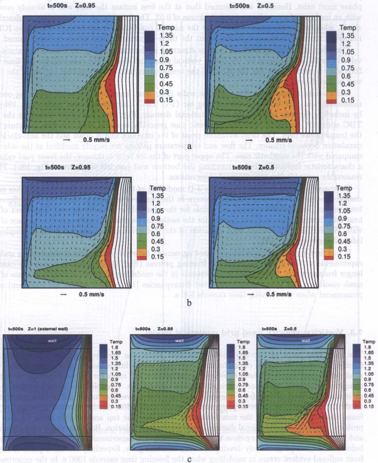
Fig. 10. Temperature and velocity fields at 500 s after freezing starts, calculated (ICE3D) for three types of thermal boundary conditions: adiabatic (a), non-adiabatic 1-TBC (b), non-adiabatic 3-TBD (c). Vertical cross-section at the side wall (left) and centre plane (right); T_A = 10^\circ\text{C} , T_c = -10^\circ\text{C}
